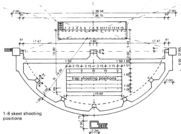
③ Combined trap and skeet shooting range
